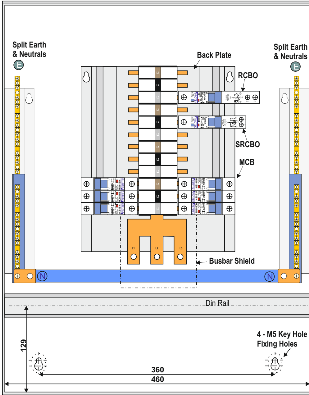
Plan View
